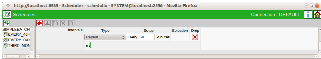
Figure 16.4: Repeat Driver
