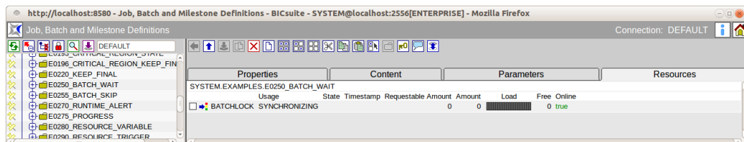
Figure 12.8: Folder resources
