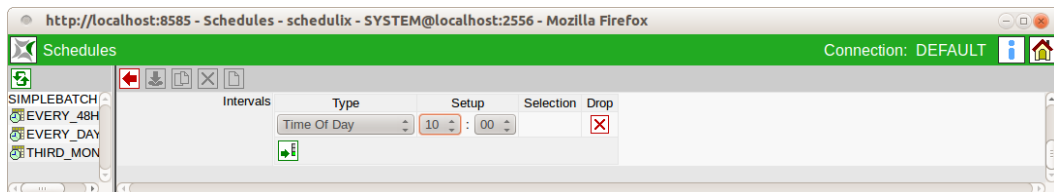
Figure 16.4: Repeat Driver
