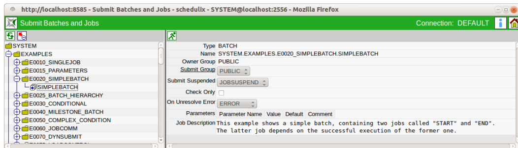
Figure 17.2: Submit navigation
