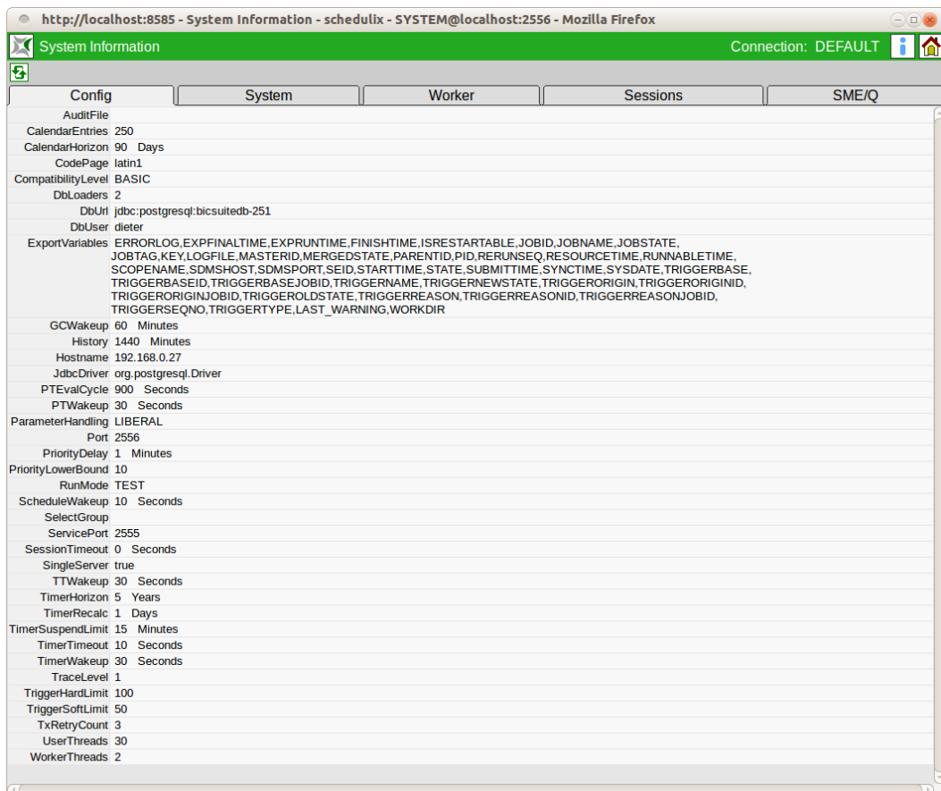
Figure 22.1: System Information
