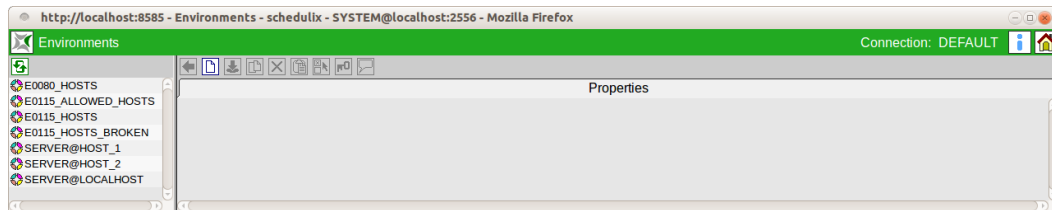
Figure 9.2: Environment navigator
