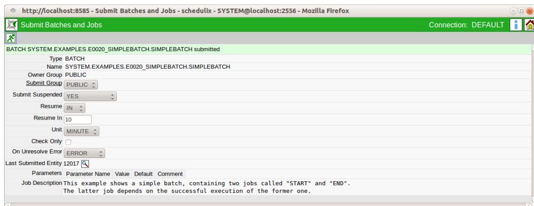
Figure 17.3: Submit editor
