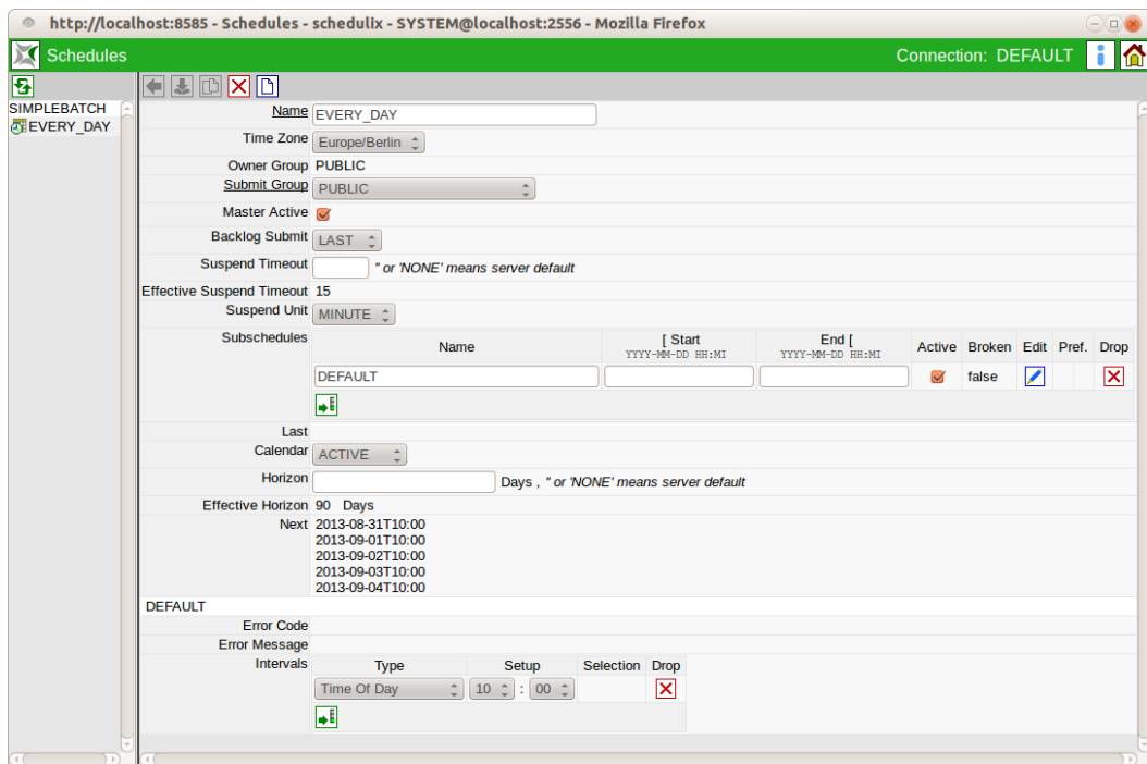
Figure 16.1: Time Scheduling
