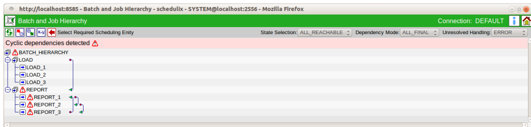
Figure 12.41: Cyclic dependencies
