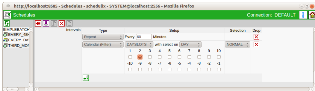
Figure 16.14: Calendar Filter
