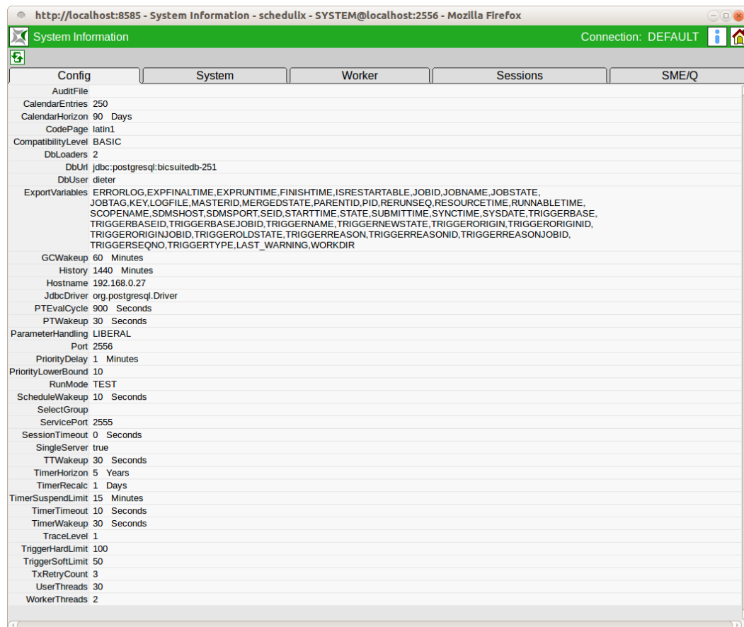
Figure 22.2: System configuration
