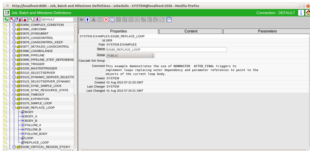
Figure 12.5: Folder properties
