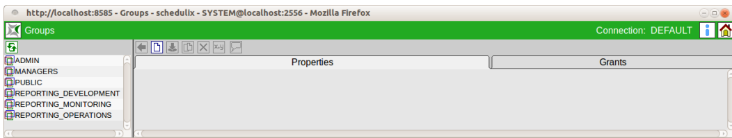
Figure 15.1: Group management
