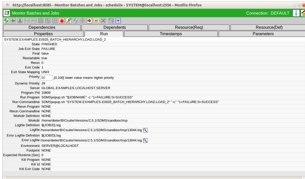
Figure 20.7: Details mask for jobs
