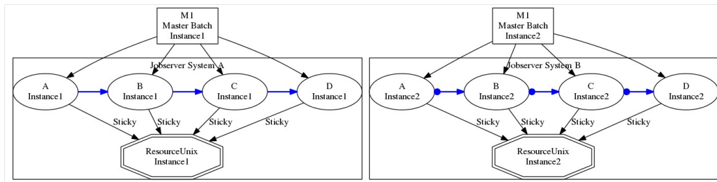
Figure 13.29: Example of load distribution with Sticky Handling
