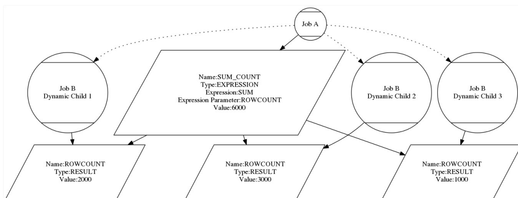
Figure 13.33: Example using Expression parameters
