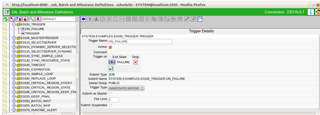
Figure 13.36: Batches and Jobs; Trigger Details tab
