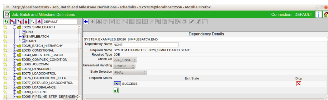
Figure 13.23: Batches and Jobs; Dependency Details
