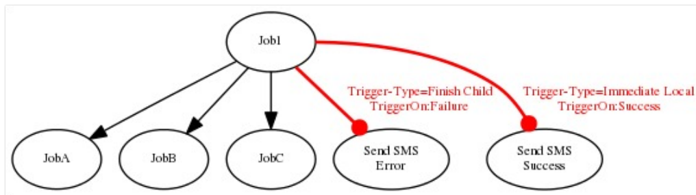
Figure 13.41: Example of a Finish Child Trigger
