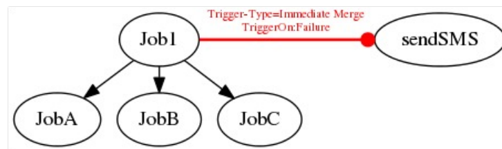
Figure 13.37: Example of an Immediate Merge trigger
