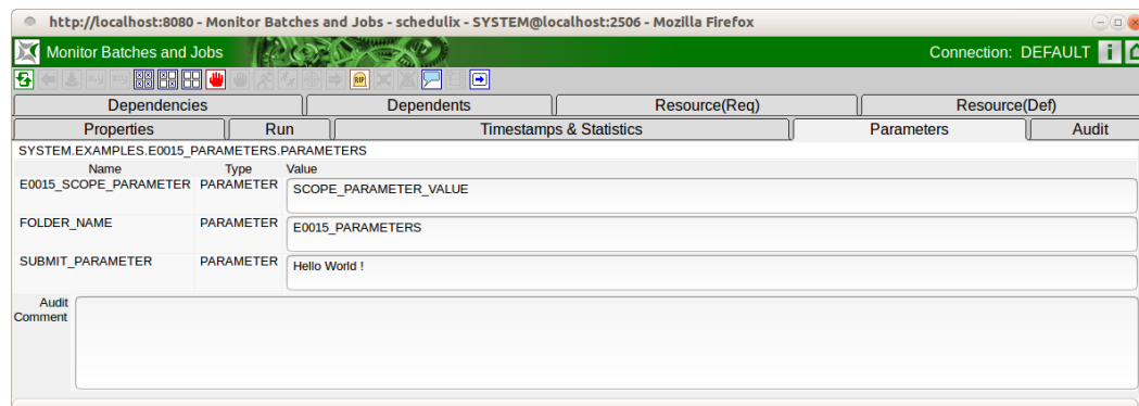
Figure 20.21: Batch and job parameters
