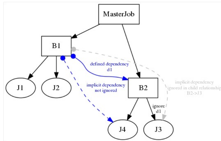
Figure 13.19: Example of Ignored Dependencies
