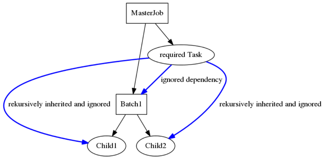
Figure 20.14: Example of a Recursive Ignore
