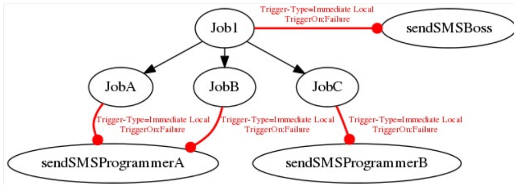
Figure 13.38: Example of an Immediate Local trigger
