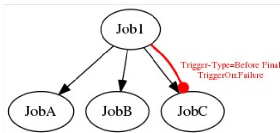
Figure 13.39: Example of a Before Final Trigger
