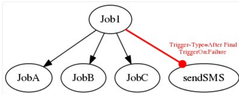
Figure 13.40: Example of an After Final Trigger
