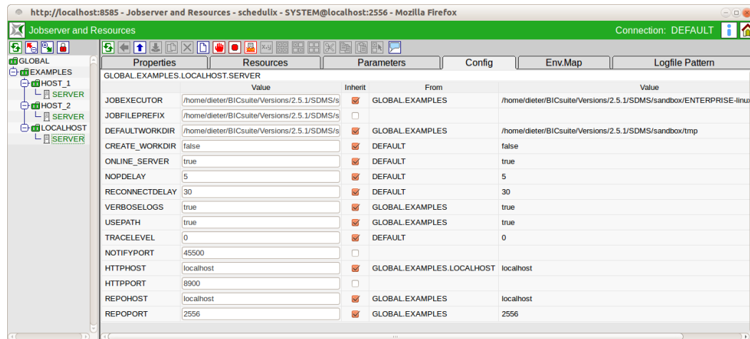
Figure 12.10: Jobserver and scope configuration
