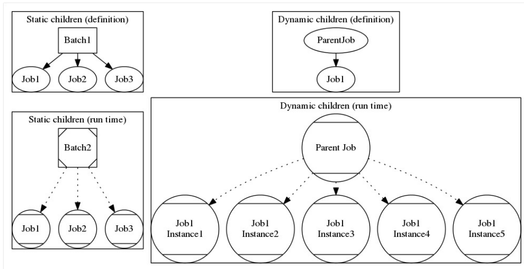
Figure 13.17: Static and dynamic children
