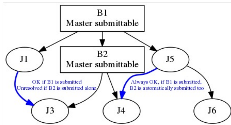
Figure 13.24: Example for Unresolved Handling
