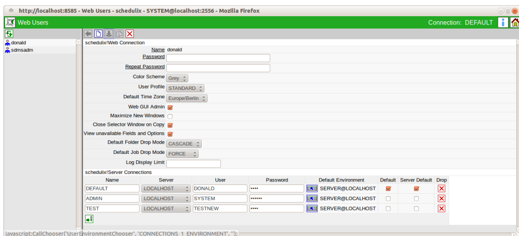
Figure 14.1: User management for the Web front end
