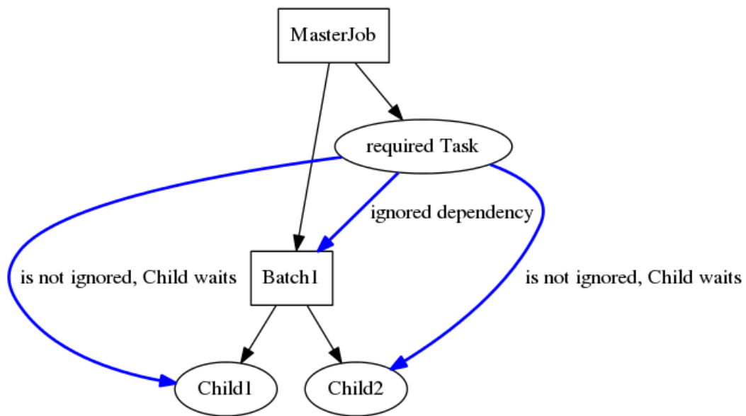
Figure 20.15: Example of a Job Only Ignore
