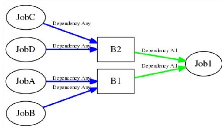
Figure 13.22: Example of Dependency Modes
