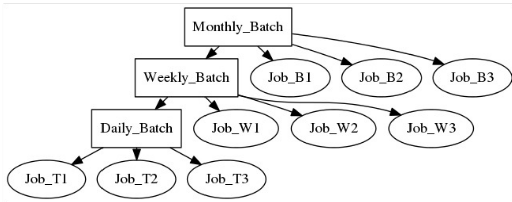
Figure 13.11: Examples of batches
